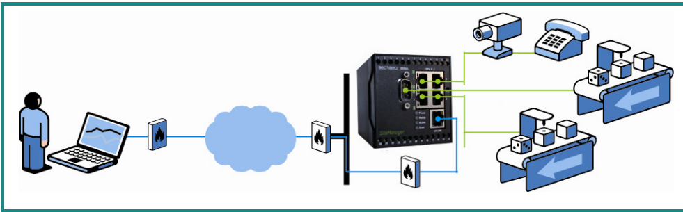
Figure 1 - System overview
